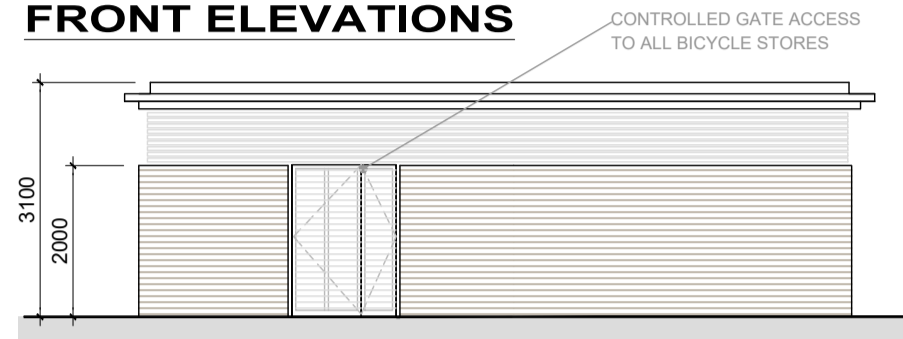
Bicycle & Bin Store - Type 1A
