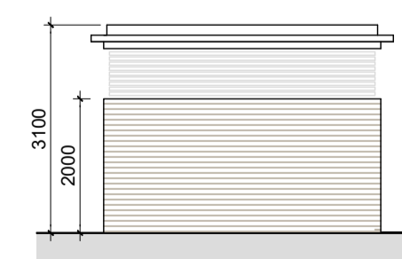
Bicycle & Bin Store Types 1C, 3A, 3B, 4A
