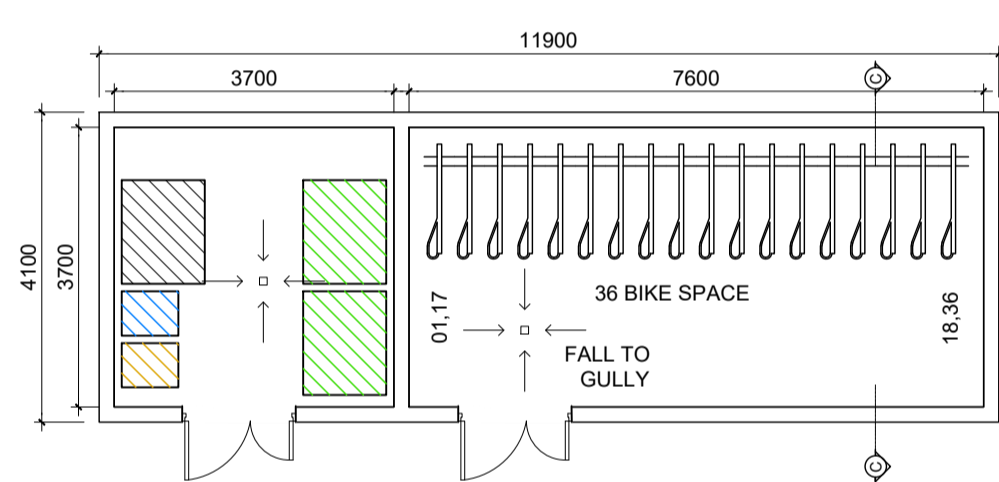
Bin Store - Type 4A
