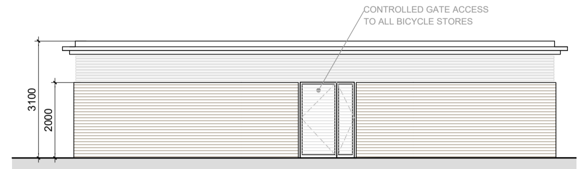
Bicycle & Bin Store - Type 1B
