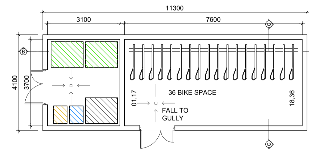
Bin / Bike Store - Type 4B
