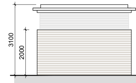
Bin Store - Type 2
