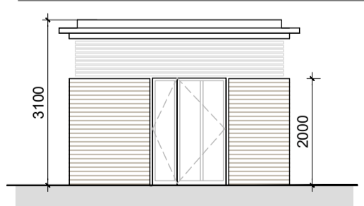
Bicycle & Bin Store Types 1A, 1B, 1D, 3B, 4B (Mirrored where applicable)
