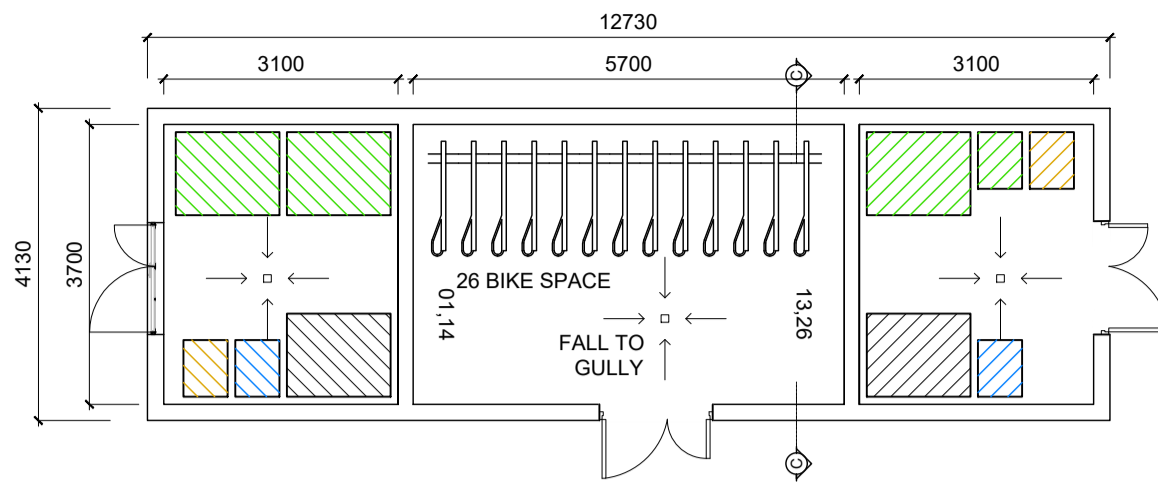
Bin / Bike Store - Type 1B
