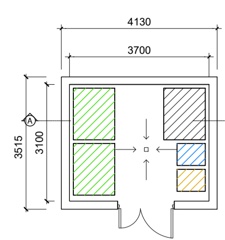
Bin Store - Type 2
