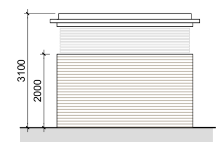
Bicycle & Bin Store Types 2
