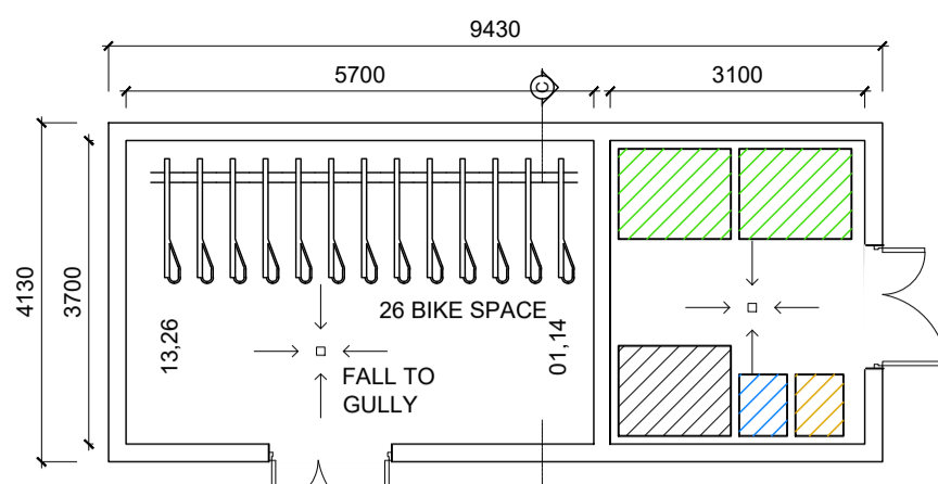
Bin / Bike Store - Type 1A
