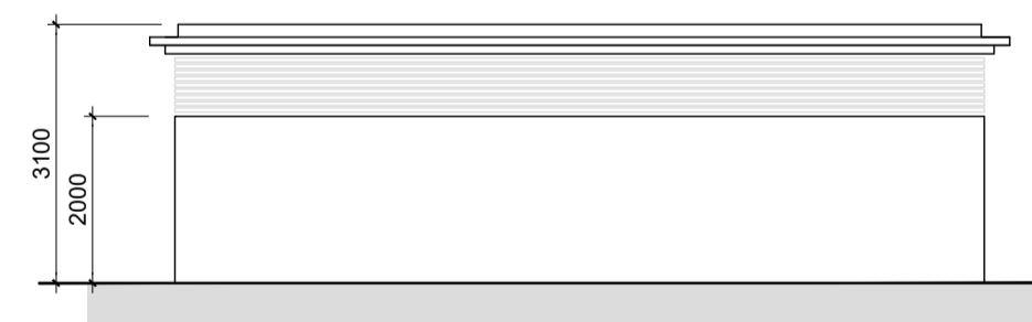
Bicycle & Bin Store - Type 3B
