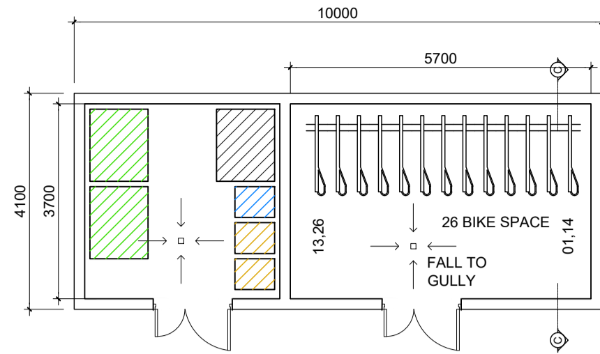
Bin / Bike Store - Type 1C
