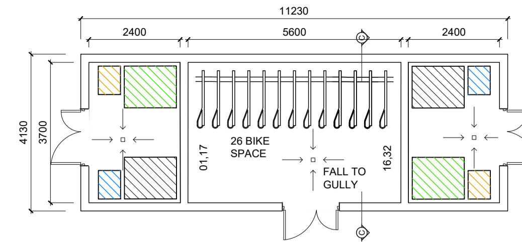
Bin / Bike Store - Type 1D
