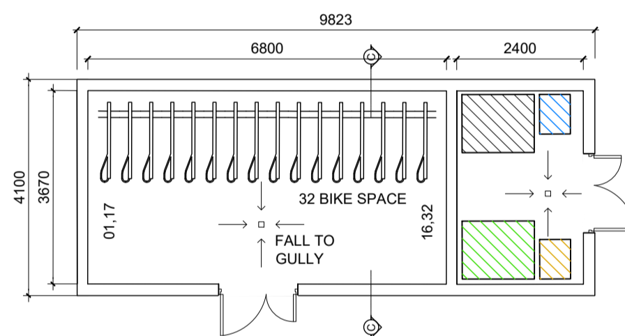
Bin / Bike Store - Type 3B
