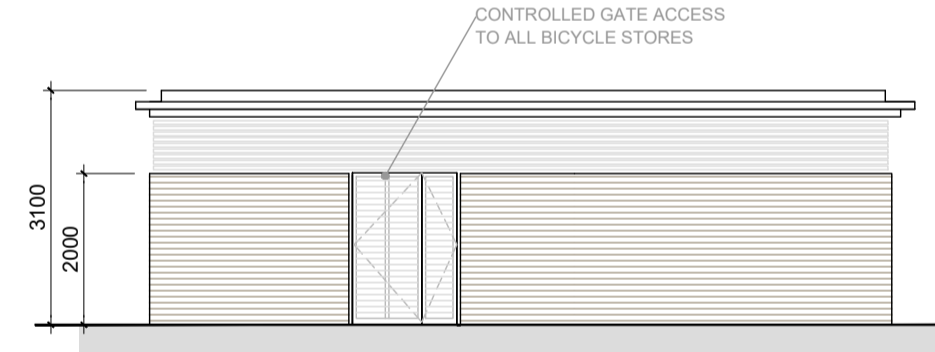
Bicycle & Bin Store - Type 3B
