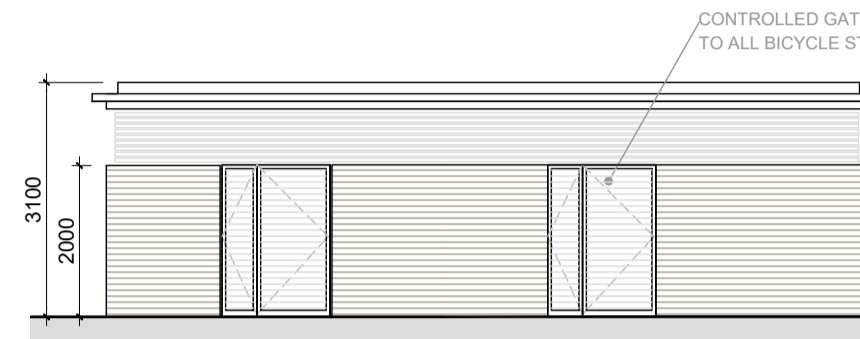
Bicycle & Bin Store - Type 1C
